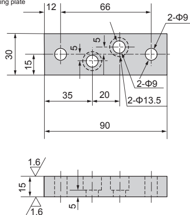
2. Kleine Montageplatte 2. Small mounting plate
