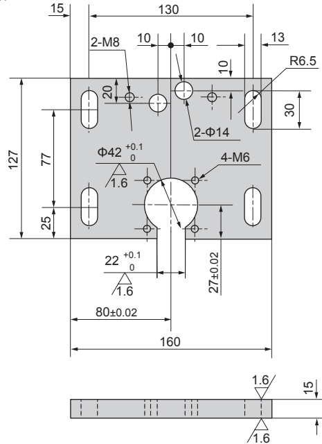
2. Kleine Montageplatte 2. Small mounting plate
